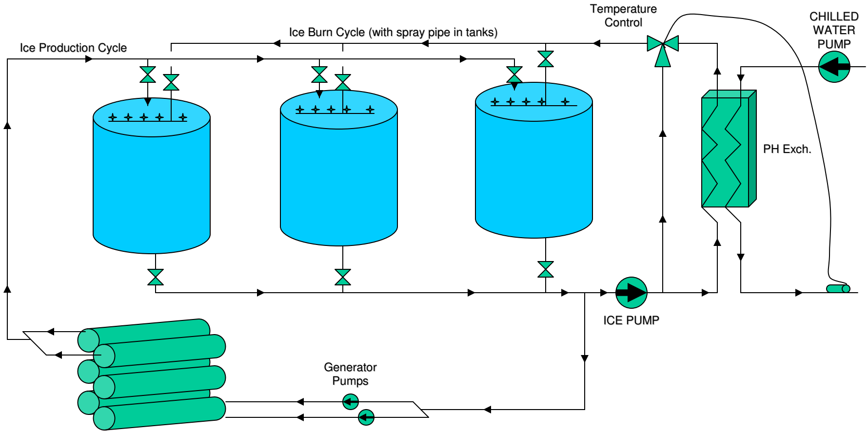
FLOW-ICE® ----General Schematic
